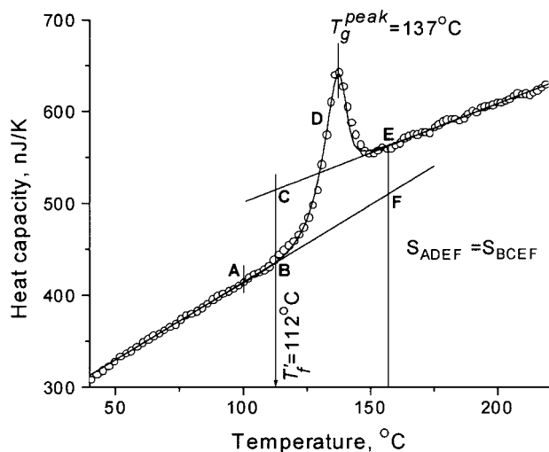
Figure 2. Calorimetric curve for 80 nm thick polystyrene on platinum, scanning rate 25 K/ms. Values of T_g^{\text{peak}} and T_f' are shown. To calculation of T_f' : points A and E lie on the linear part of the curve.
