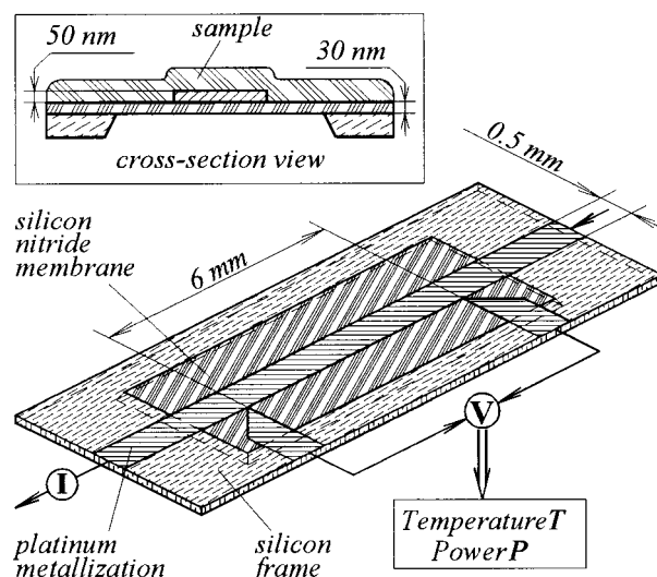
Figure 1. MEMS-based calorimetric sensor for TDSC (not to scale).
