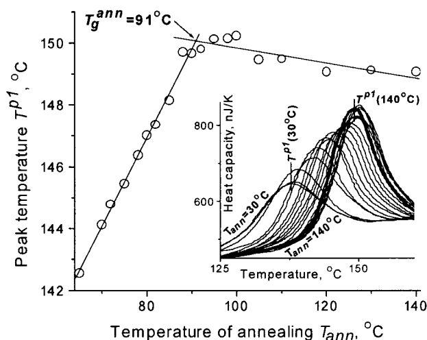
Figure 3. Calculation of T_g^{\text{ann}} . The sample is the same as in Figure 2. The set of the first run calorimetric curves after annealing at different temperatures is shown in the inset.
